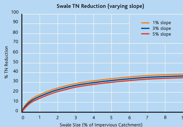
Figure 2. TN reduction by a swale in Melbourne as slope varies (0.25m vegetation height)
