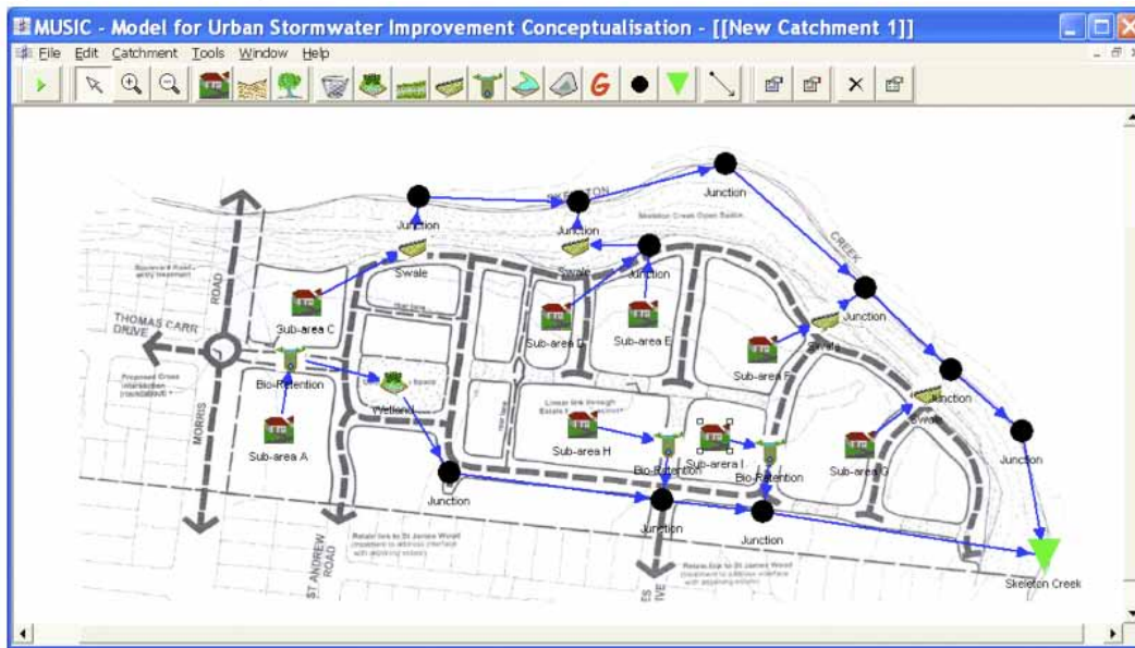
Figure 31. The structure of a MUSIC model to evaluate stormwater treatments using raingardens in a typical residential development
