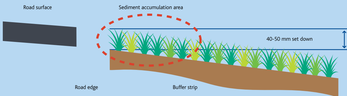
Figure 3 Typical buffer strip arrangement
