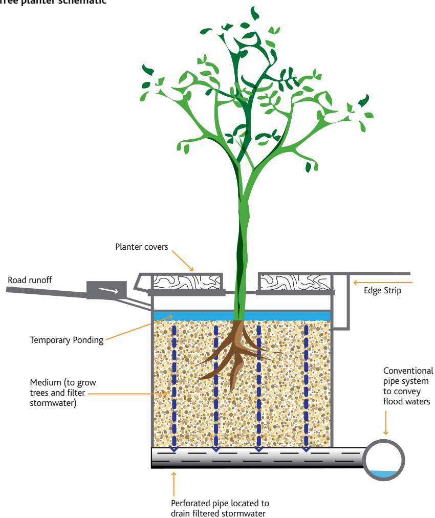
Figure 27. Tree planter schematic
