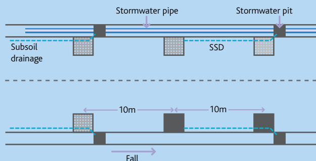
Figure 4. Typical street layout for raingarden tree pit – roadside of the kerb
