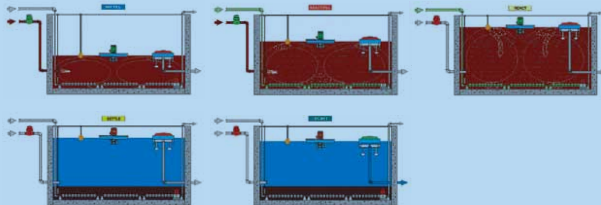
Figure 1 Schematic of SBR system
