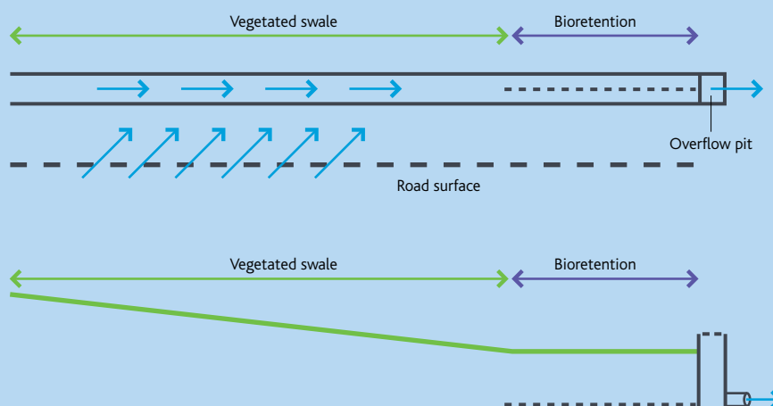
Figure 3: typical swale raingarden system adjacent to roadside – plan and section drawing
