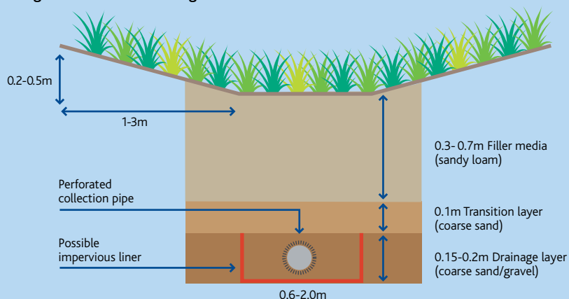
Figure 2: Typical swale raingarden – section drawing
