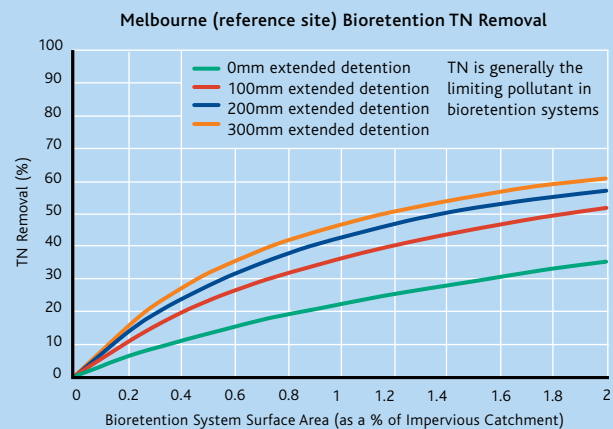
Figure 1: TN removal by Raingardens in Melbourne
