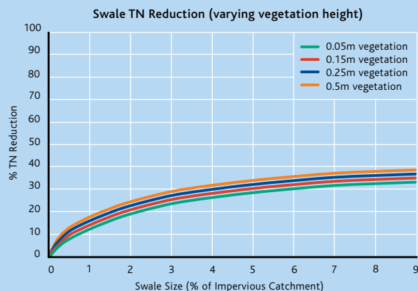
Figure 1. TN reduction by a swale in Melbourne as vegetation varies (3% slope)
