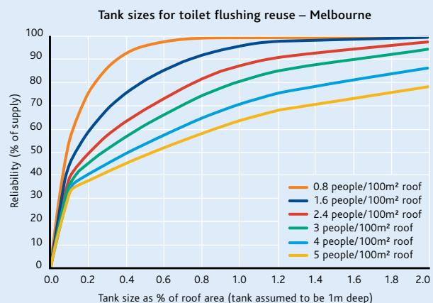
Figure 1: Rainwater tank sizing curve for toilet flushing in Melbourne
