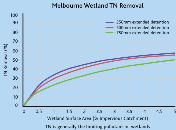
Figure 1 Sizing curve for wetlands in Melbourne
