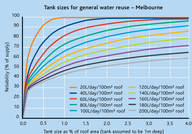
Figure 1: General use tank sizing curve for Melbourne
