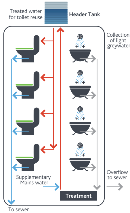
Figure 11. Greywater system within a multi-storey residential development
