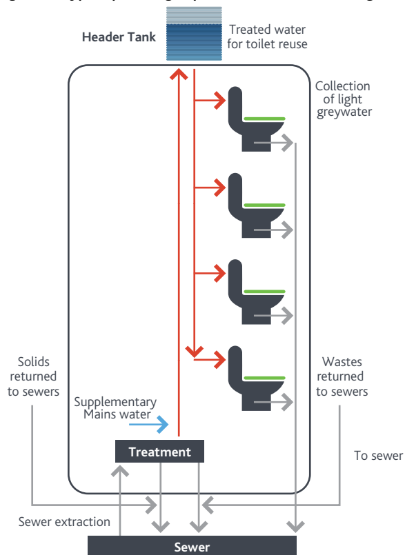
Figure 15. Typical plumbing requirements for sewer mining within high rise development
