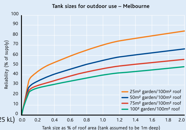
Figure 2: Rainwater tank sizing curve for outdoor use in Melbourne
