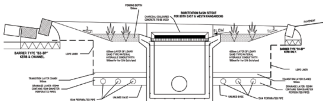
Figure 33. Section detail of Raingarden
